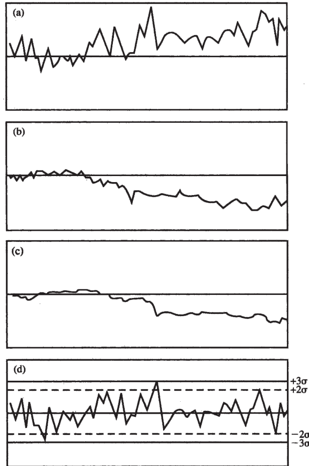
FIGURE 15.10 (a) Disturbance N_t , (b) feedback control action X_t , (c) compensation of the disturbance Y_t , and (d) resulting deviation \varepsilon_t from the target value.
