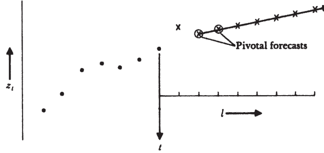
FIGURE 5.3 Eventual forecast function for an IMA(0, 2, 3) process.
