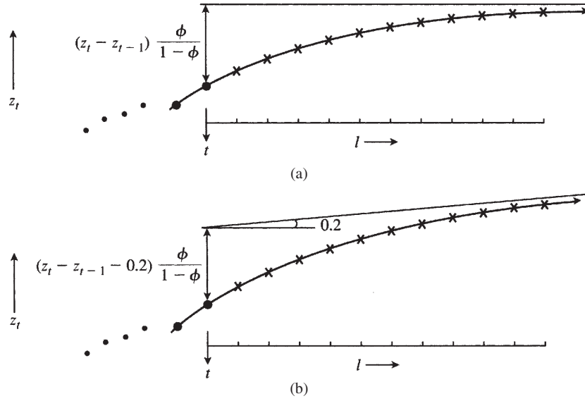
FIGURE 5.10 Forecast functions for two (1, 1, 0) processes. (a) Forecasts of a (1, 1, 0) process (1 - 0.8B)\nabla z_t = a_t . (b) Forecasts of a (1, 1, 0) process (1 - 0.8B)(\nabla z_t - 0.2) = a_t .
