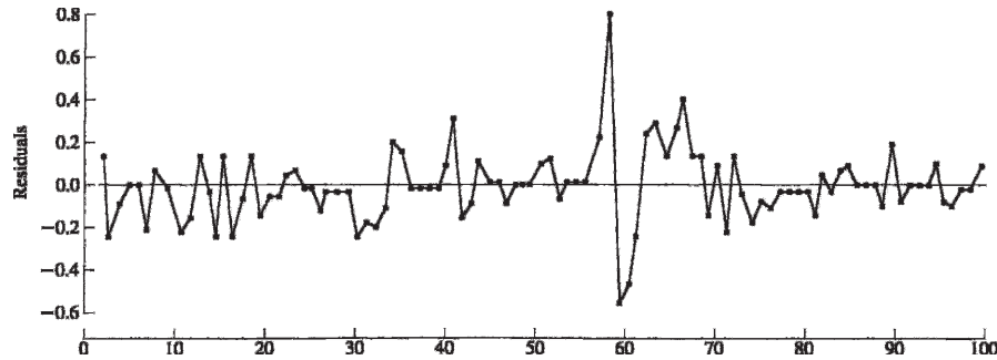
FIGURE 13.2 First 100 residuals from the ARIMA(1, 1, 0) model fitted to Series C.
