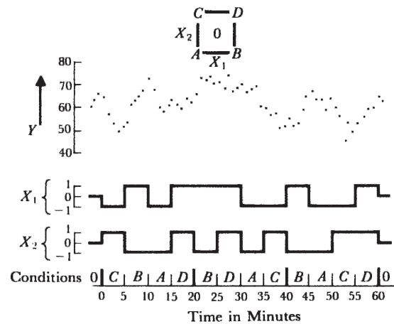
FIGURE 12.8 Data for simulated two-input example (Series K).
