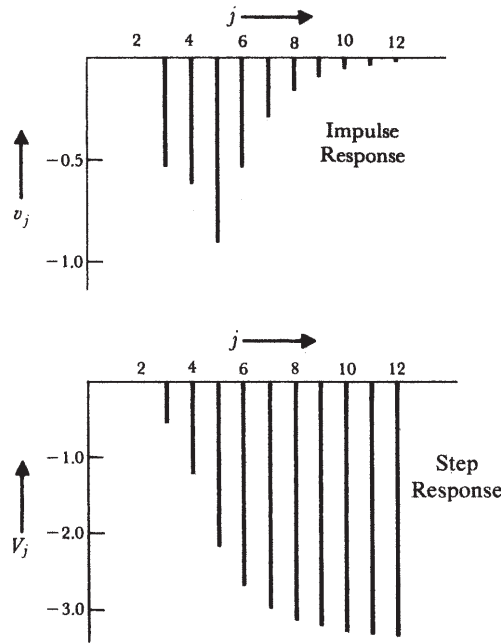
FIGURE 12.6 Impulse and step responses for transfer function model (1 - 0.57B)Y_t = -(0.53 + 0.37B + 0.51B^2)X_{t-3} fitted to coded gas furnace data.
