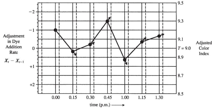
FIGURE 15.8 Manual adjustment chart putting into effect discrete integral plus proportional control.
