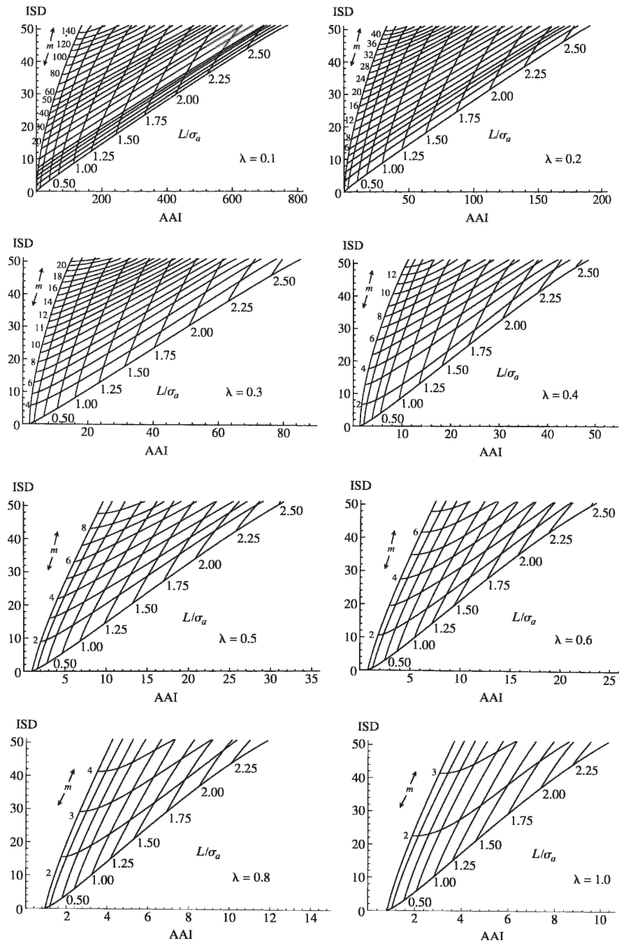
FIGURE 15.13 Charts for \lambda = 0.1, 0.2, 0.3, 0.4, 0.5, 0.6, 0.8, and 1.0 showing AAIs and ISDs obtained from various choices of L/\sigma_a and m .
