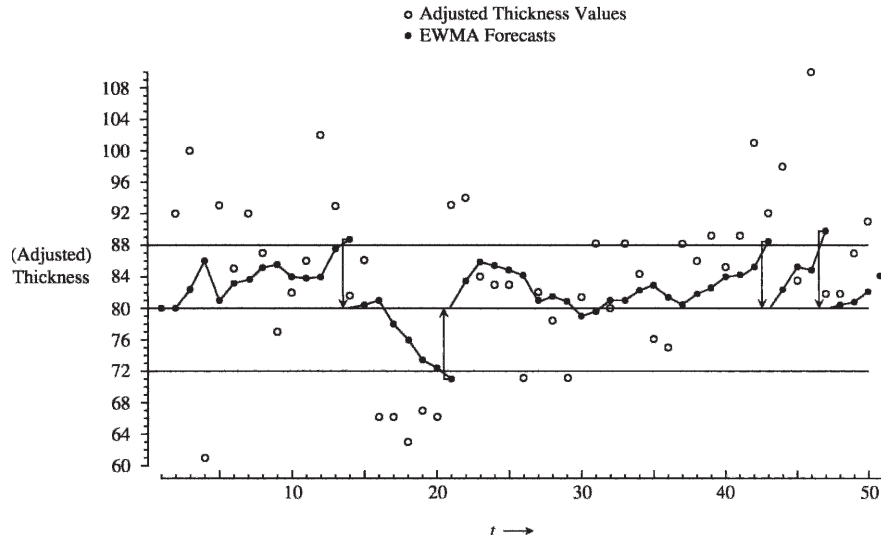
FIGURE 15.11 Bounded adjustment chart: the open circles are the thickness deviations \varepsilon_t (after adjustment), the closed circles are their EWMA forecasts \hat{\varepsilon}_{t-1}(1) of these deviations.
