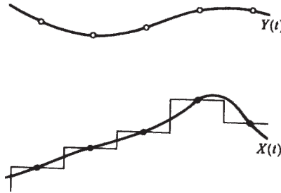
FIGURE 11.11 Replacement of continuous input by pulsed input.
