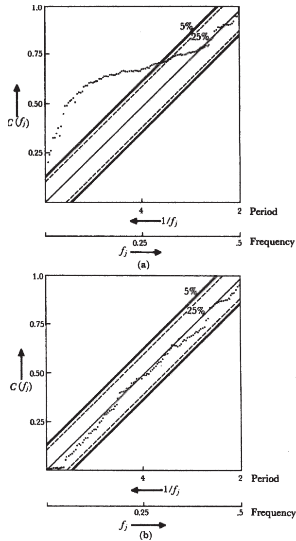
FIGURE 8.3 Series C: cumulative periodograms of residuals from best-fitting models (a) of order (0, 1, 1) and (b) of order (0, 2, 2).
