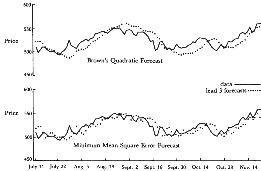
FIGURE A5.2 IBM stock price series with comparison of lead 3 forecasts obtained from best IMA (0, 1, 1) model and Brown's quadratic forecast for a period beginning July 11, 1960.
