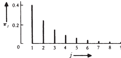
FIGURE 4.7 The \pi weights for an IMA process of order (0, 1, 1) with \lambda = 1 - \theta = 0.4 .
