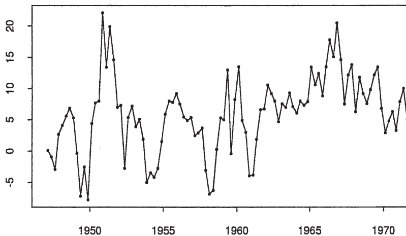
(b) z_{2t} : Changes in Business Inventories Series
