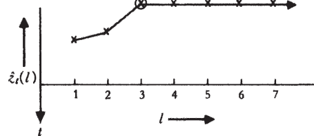
FIGURE 5.8 Forecast function for an IMA(0, 1, 3) process.
