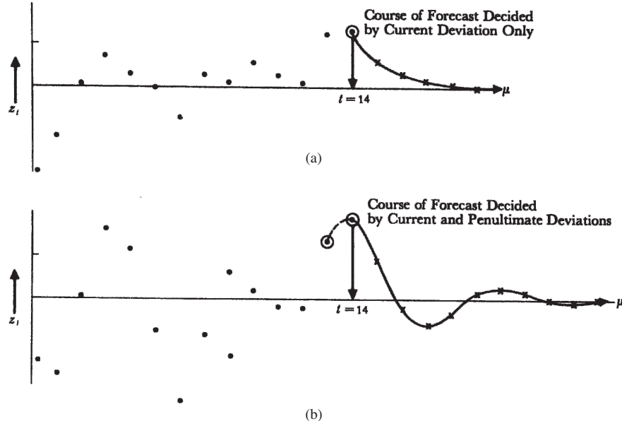
FIGURE 5.9 Forecast functions for first- and second-order autoregressive processes. (a) A sample from a first-order autoregressive process (1 - 0.5B) \tilde{z}_t = a_t , and forecast function from origin t = 14 . (b) A sample from a second-order autoregressive process (1 - 0.75B + 0.50B^2) \tilde{z}_t = a_t , and forecast function from origin t = 14 .
