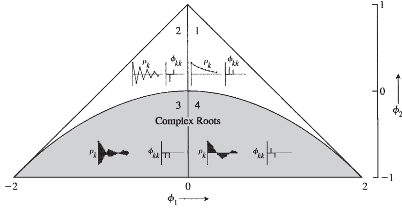
FIGURE 3.2 Typical autocorrelation and partial autocorrelation functions \rho_k and \phi_{kk} for various stationary AR(2) models. (From [270].)
