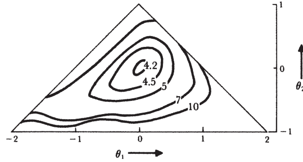
FIGURE 7.6 Contours of S(\hat{\phi}_\theta, \theta) plotted over the admissible parameter space for the \theta 's.
