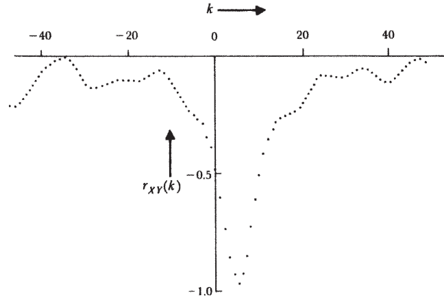
FIGURE 12.4 Estimated cross-correlation function between input and output for coded gas furnace data read at 9-second intervals.
