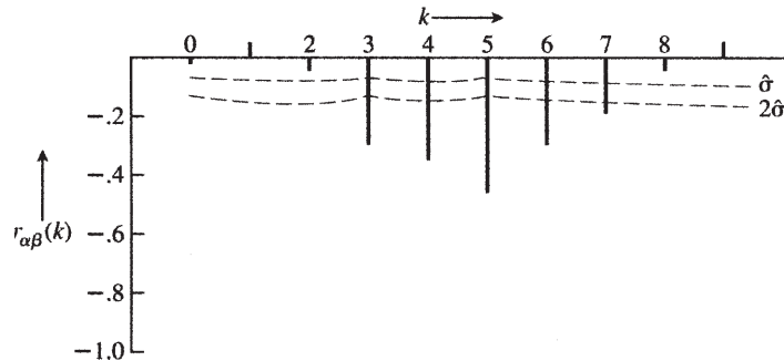
FIGURE 12.5 Estimated cross-correlation function for coded gas furnace data after prewhitening.
