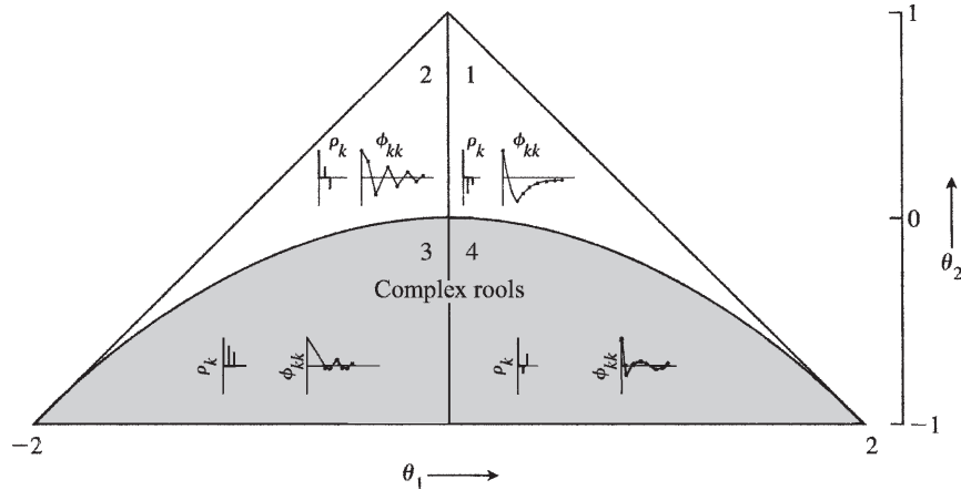
FIGURE 3.9 Autocorrelation and partial autocorrelation functions \rho_k and \phi_{kk} for various MA(2) models. (From [270].)
