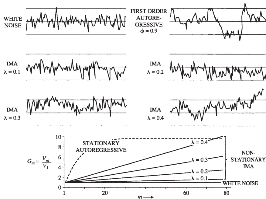
FIGURE 15.6 Realizations of white noise, autoregressive, and IMA(0, 1, 1) time series with theoretical variograms.
