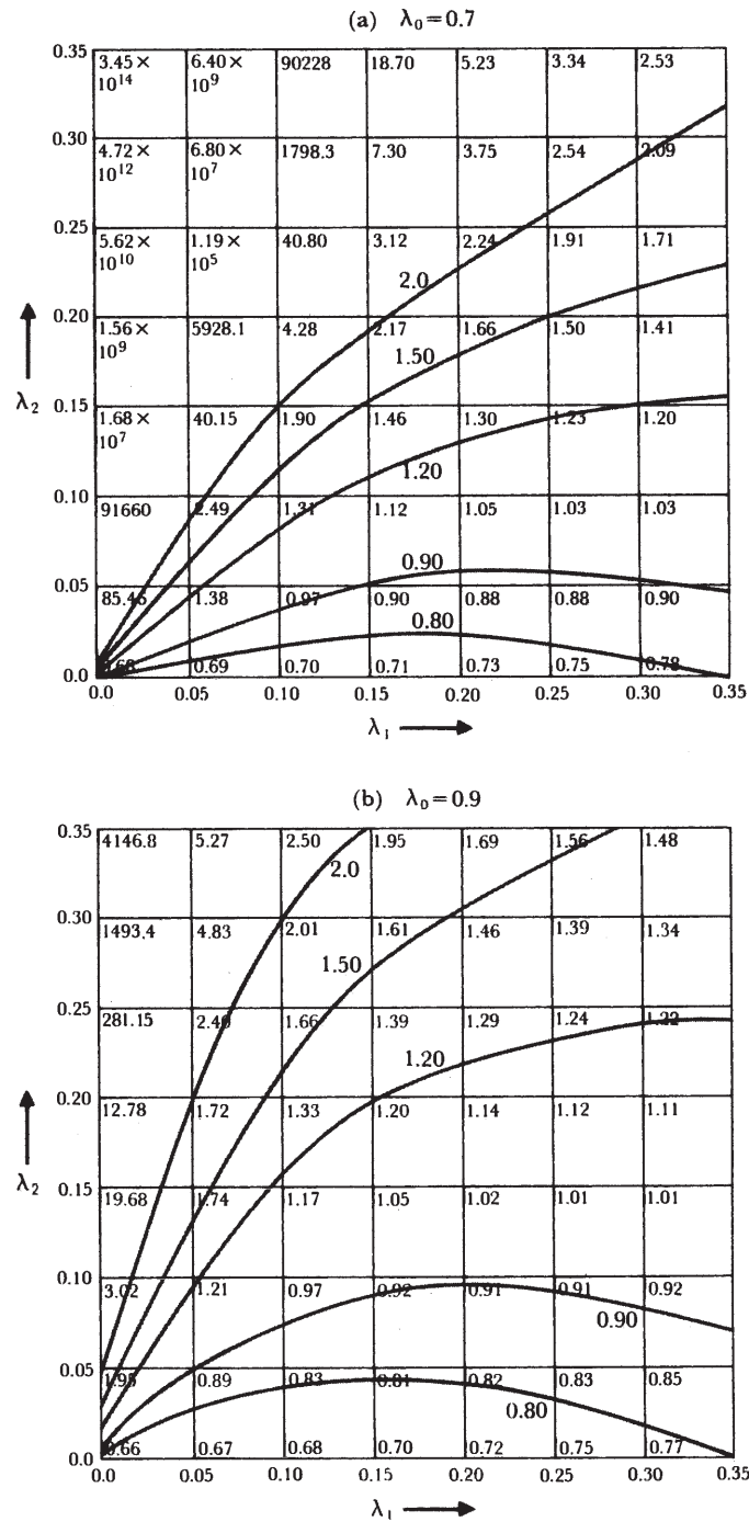
FIGURE 8.1 Sum-of-squares grids and contours for Series B' for extended model of order (0, 3, 3).
