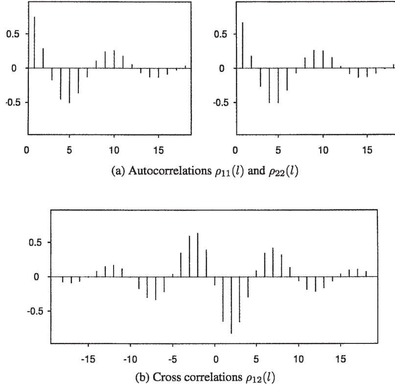
FIGURE 14.1 Theoretical autocorrelations and cross correlations, \rho_{ij}(l) , for the bivariate AR(1) process example: (a) autocorrelations \rho_{11}(l) and \rho_{22}(l) and (b) cross correlations \rho_{12}(l) .
