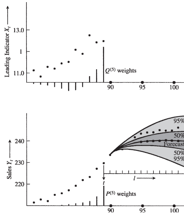
FIGURE 12.11 Forecast of sales at origin t = 89 with P and Q weights for lead 5 forecast.
