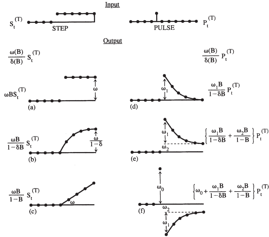
FIGURE 13.1 Responses to a step and a pulse input: (a), (b), (c) response to a step input for various simple transfer function models; (d), (e), (f) response to a pulse input for some models of interest.
