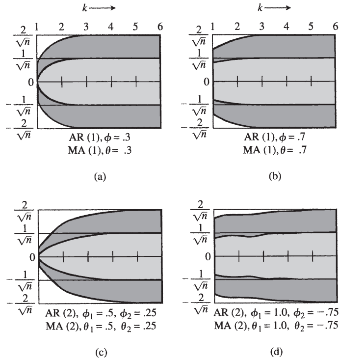
FIGURE 8.2 Standard error limits for residual autocorrelations r_k(\hat{a}) .
