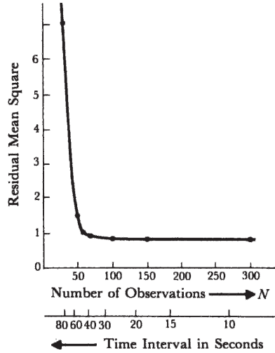
FIGURE 12.7 Mean square error at the output for various choices of sampling interval.
