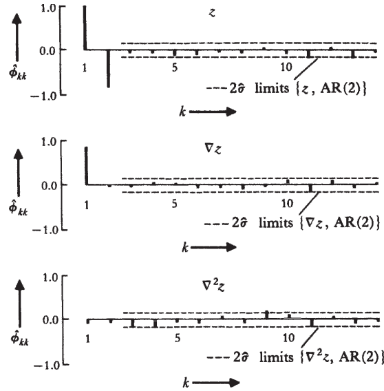
FIGURE 6.5 Estimated partial autocorrelations of various differences of Series C.
