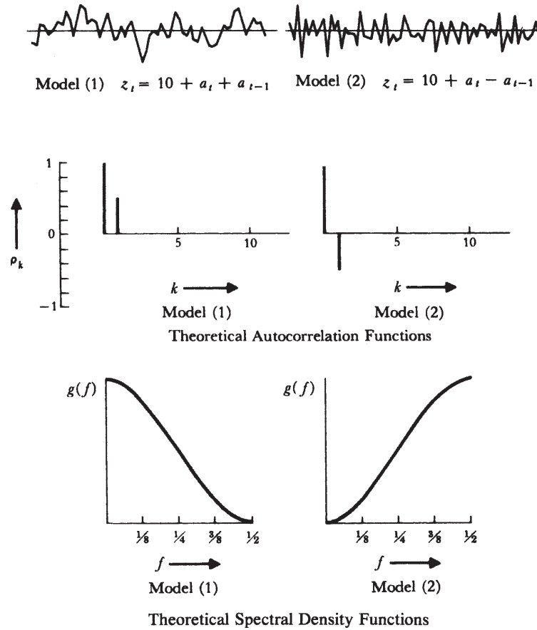
FIGURE 2.9 Two simple stochastic models with their corresponding theoretical autocorrelation functions and spectral density functions.
